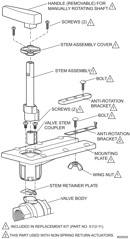
Fig. 6. Valve assembly exploded view.
