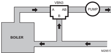
Fig. 4. Reset mixing control for discharge hot water.
