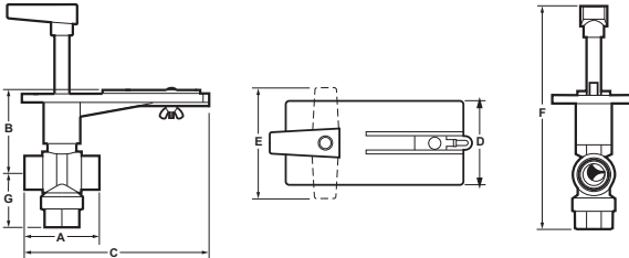
Fig. 8. VB2 dimensions in inches (mm).
