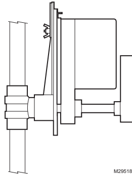
Fig. 1. Vertical valve installation.
