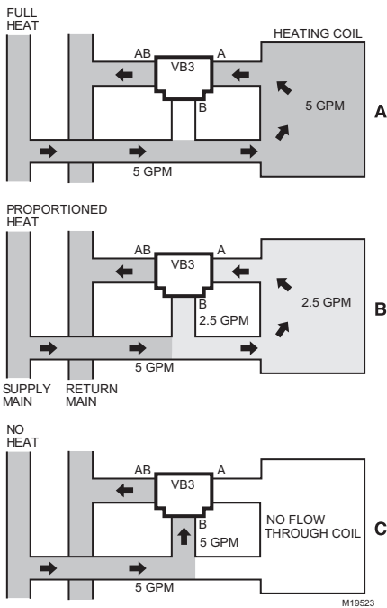
Fig. 5. Three-way mixing valve operation with coil bypass.
