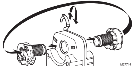
Fig. 7. SCSA Mounting
