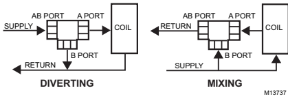
Fig. 3. Three-way ball valve flow orientation (not to scale).
